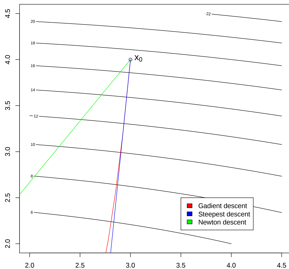
Figure 6.23: Closeup of the paths obtained by the Newton descent and other similar algorithms
