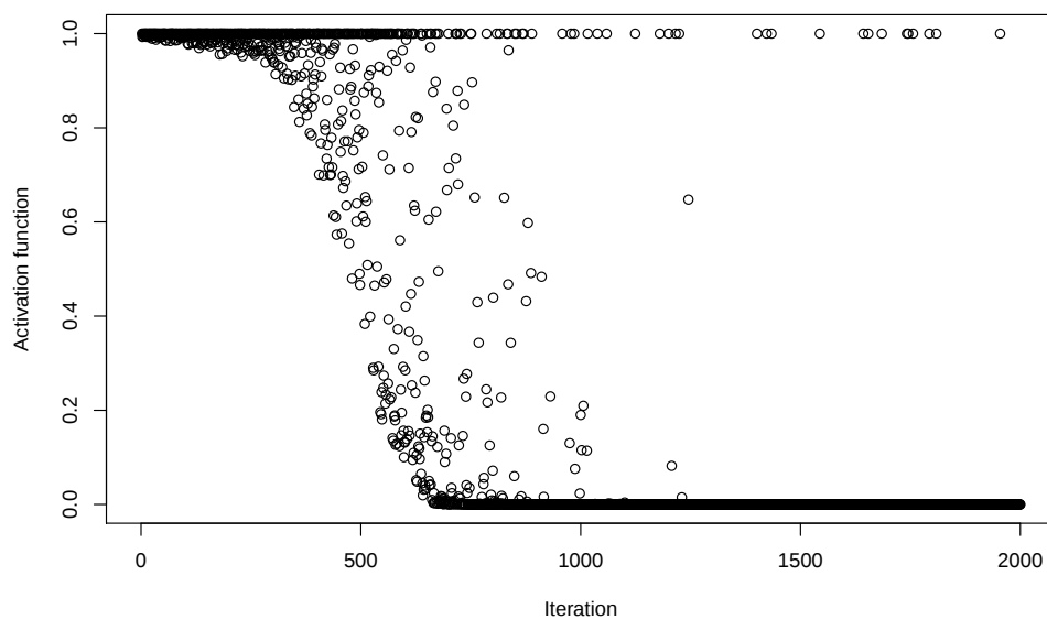
Figure 7.29: A plot of the activation function values over subsequent iterations of the algorithm.
